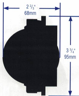
X-TD Tie-Down (compass not included)
